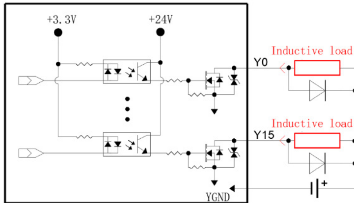
Figure 5 Wiring of inductive load
