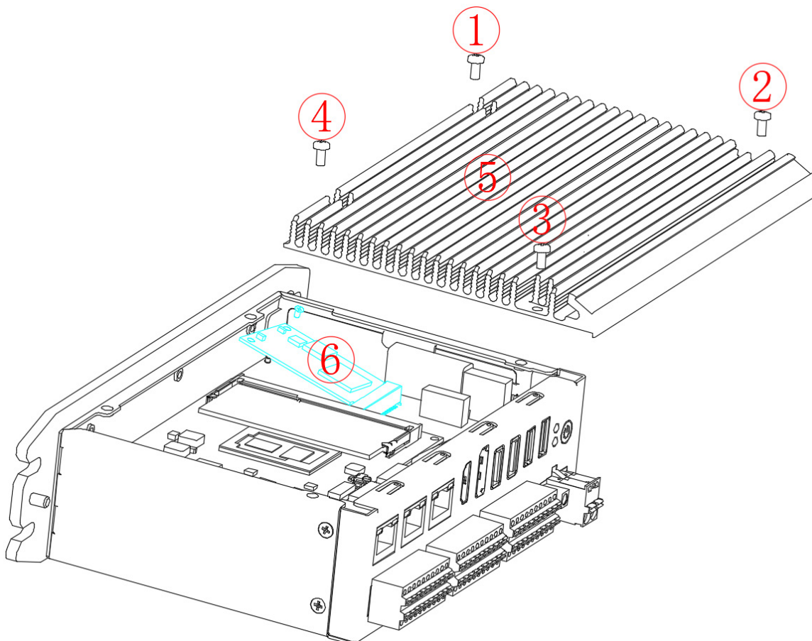
Figure 10 SSD Setup
