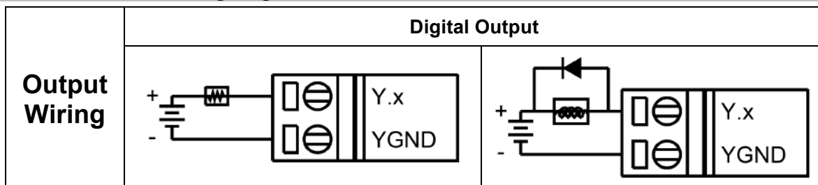
Figure 13 DO electrical wiring diagram
