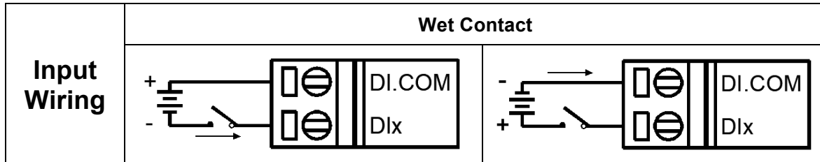
Figure 12 DI electrical wiring diagram
