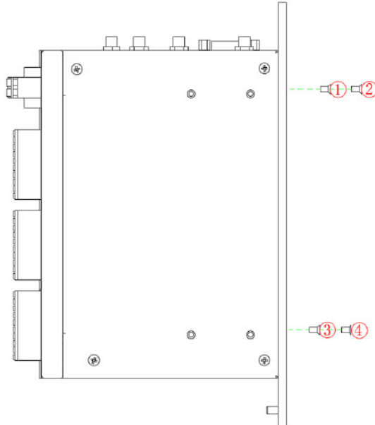
Figure 8 Attach the wall-mount part
