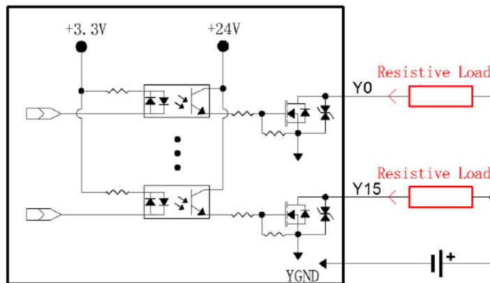
Figure 4 Wiring of resistive load
