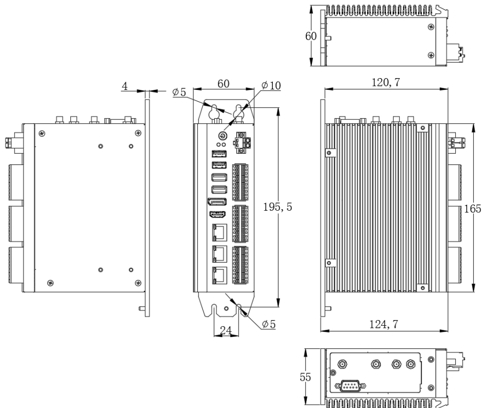
Figure 1 Dimension of NP-6118
