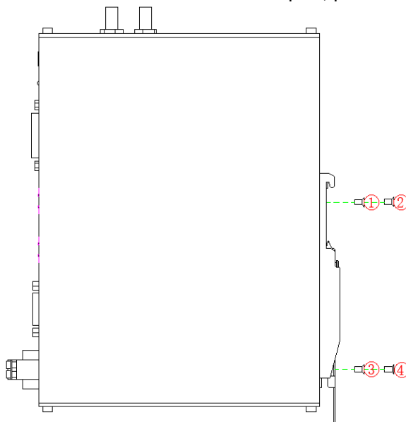
Figure 9 Attach DIN-Rail mounted part
